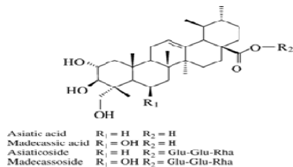
Figure 1: Asiaticoside structure
