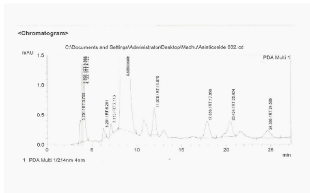
Figure 4: HPLC of Centella asiatica leaf extracts (Subhodak)
