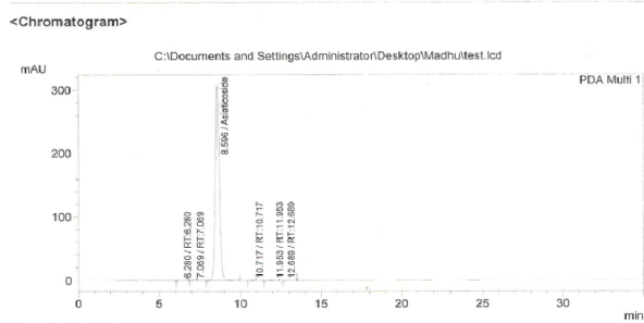
Figure 2: HPLC of standard Asiaticoside
