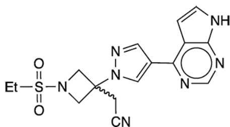
Figure 1. Structure of Baricitinib
