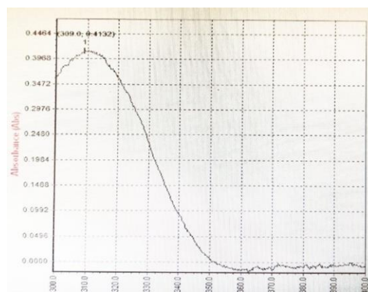
Figure 2. Determination of λmax of Baricitinib pure drug
