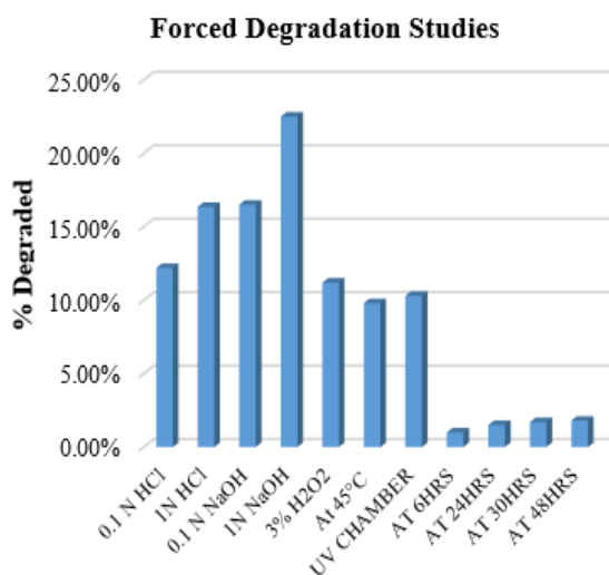
Figure 4. Forced degradation studies graph of Baricitinib.
