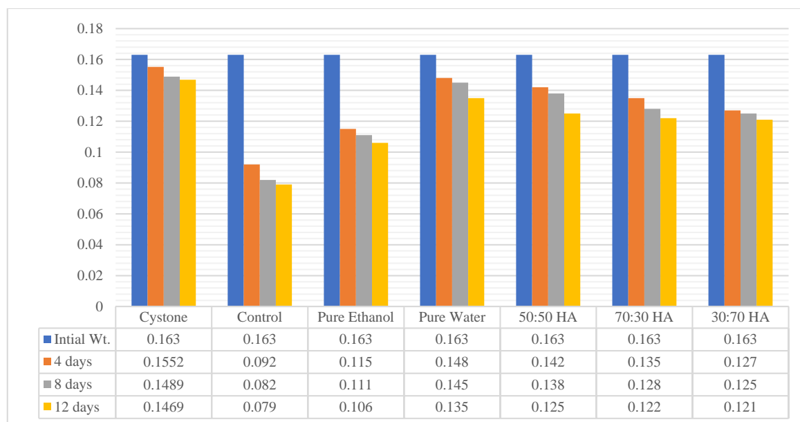
Figure 4. Percent Graphical representation of dissolution of calcium oxalate (100 mg)
