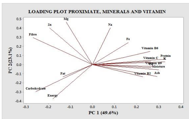
Figure 5. Principal component analysis (Loading plot) using 17 variables listed in Tables 1
