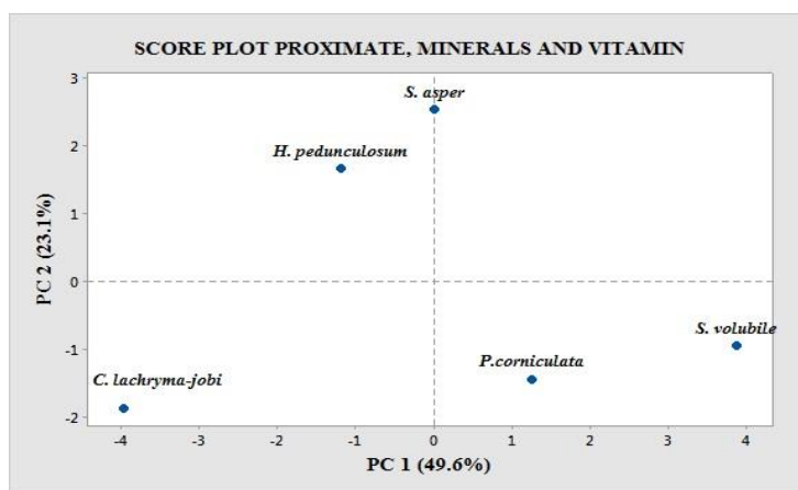
Figure 4. Principal component analysis (Score plot) using 17 variables listed in Tables 1
