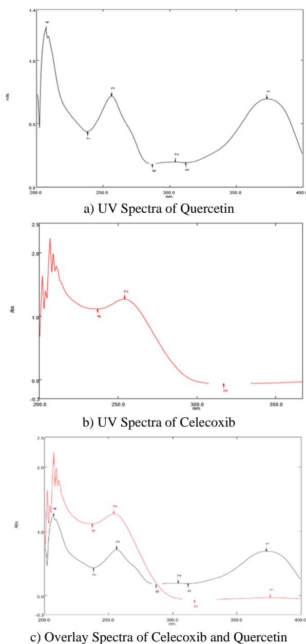
Figure 2. UV Spectra of Quercetin and Celecoxib
