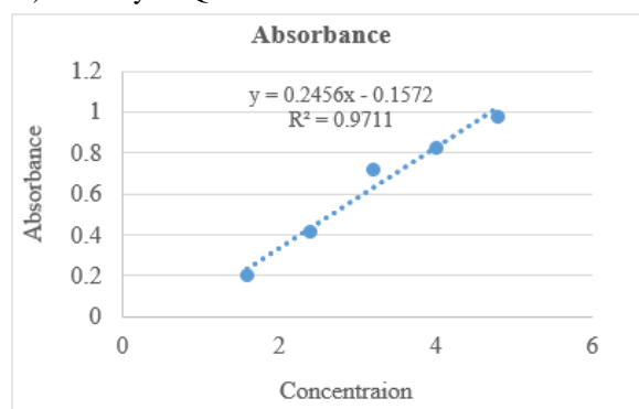
b) Linearity of Celecoxib in Simultaneous Estimation
