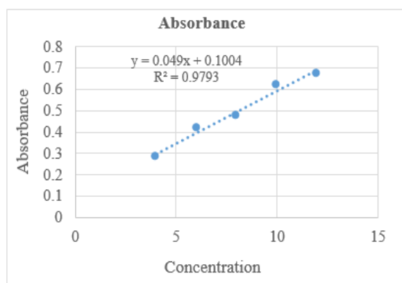
a) linearity of Quercetin in Simultaneous Estimation
